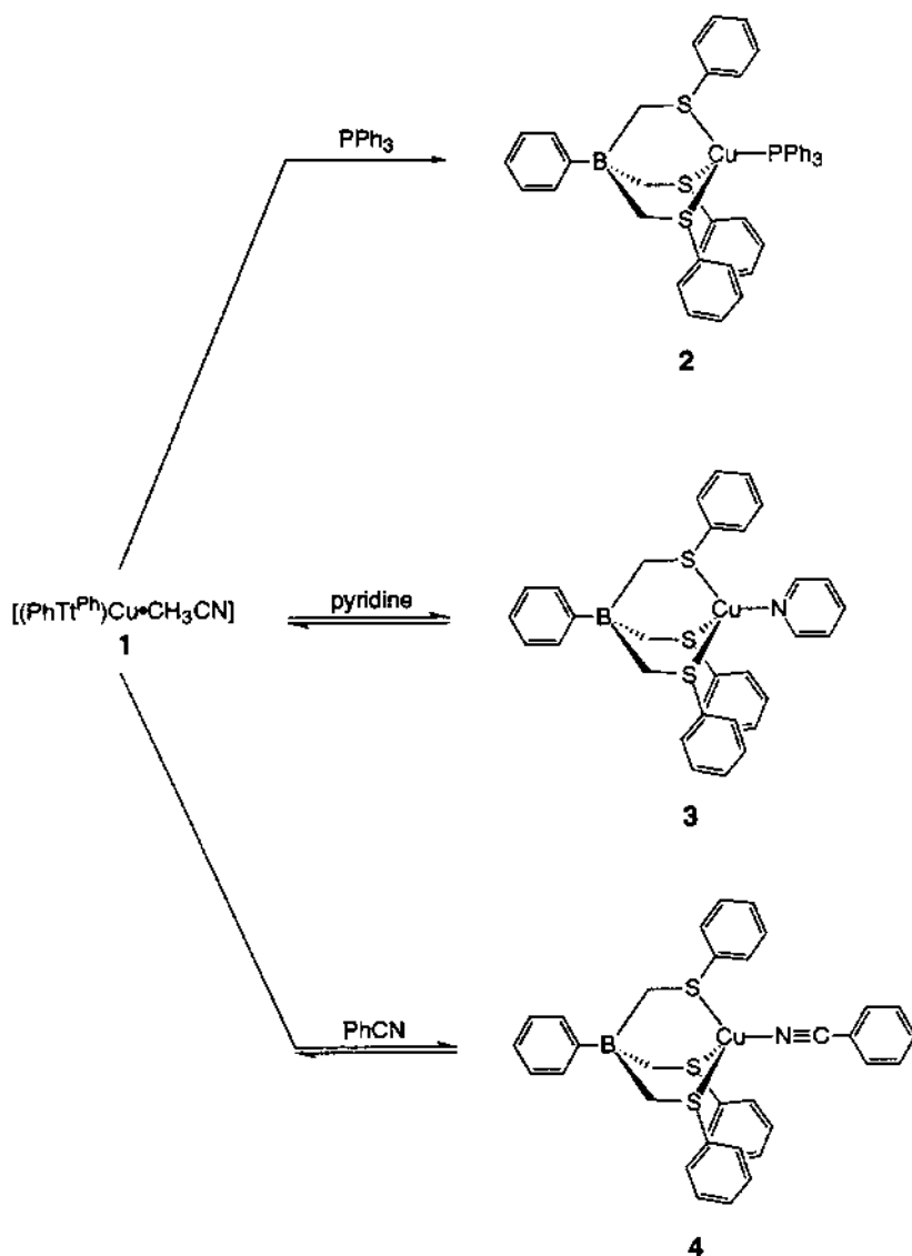
Scheme 2. Substitution reactions.
